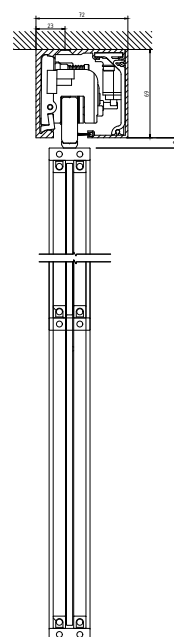
MUTO Comfort XL 150 ceiling mount
