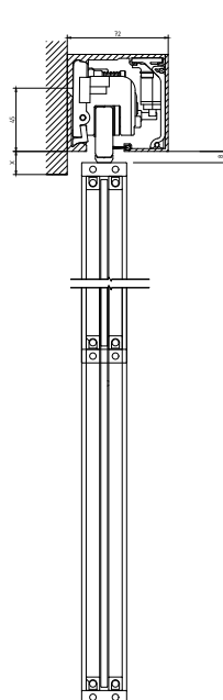
MUTO Premium XL 150 wall mounting
