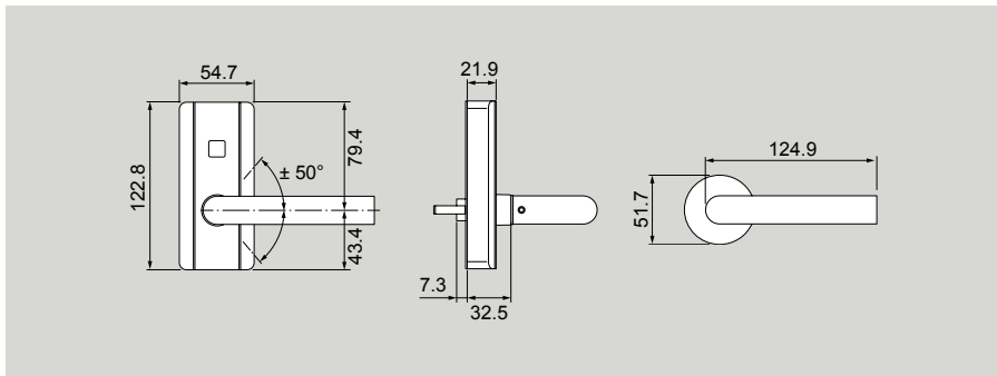
c-lever compact, standard version type 2725 54.7 x 122.8 x 21.9 mm (B x H x T)
